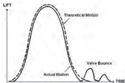
Fig.1: Theoretical compared to actual valve open curve.
