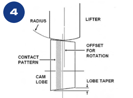
Fig.4: Correct flat tappet assembly
