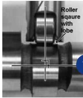
Fig.7: Correct cam-lifter angle
