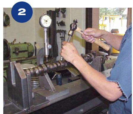
Fig.2: Straightening a camshaft
