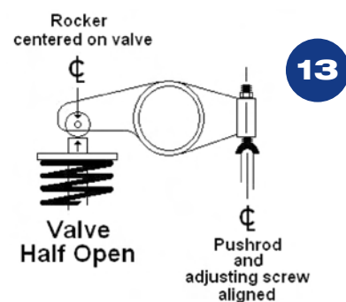
Fig.13: Correct rocker and pushrod geometry
